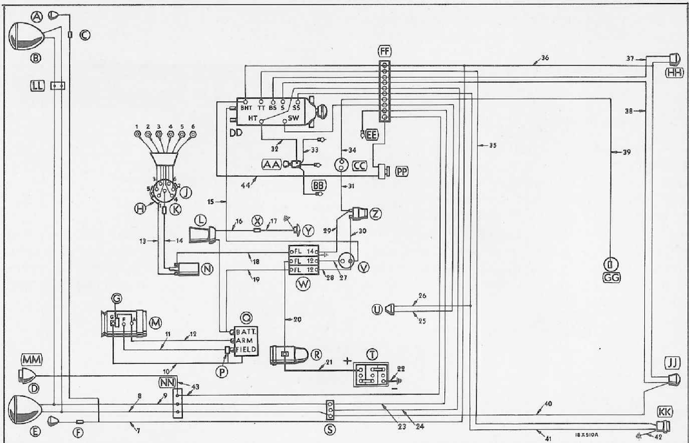
Fig. 86—Wiring Circuit Diagram (Weapons Carrier)
