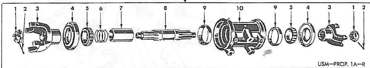
EXPLODED VIEW OF PILLOW BLOCK
