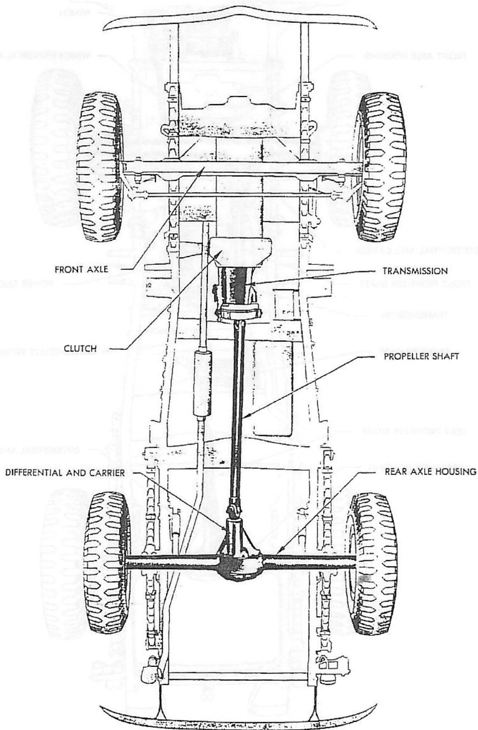
UNDERSIDE VIEW OF CHASSIS (4x2)
