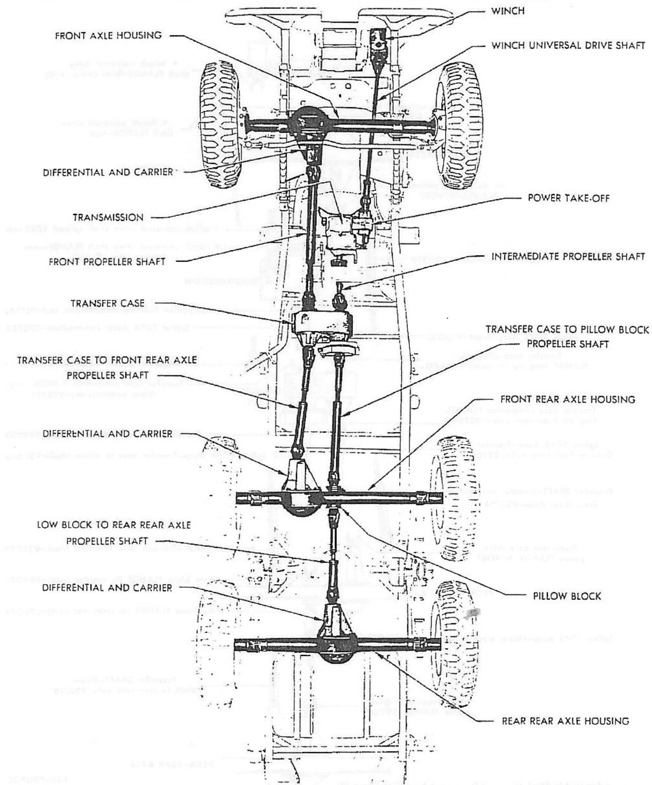
UNDERSIDE VIEW OF CHASSIS MODEL T-223 (6x6)
