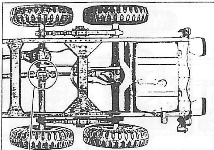
TOP VIEW OF CHASSIS MODEL T-223 (6x6)
