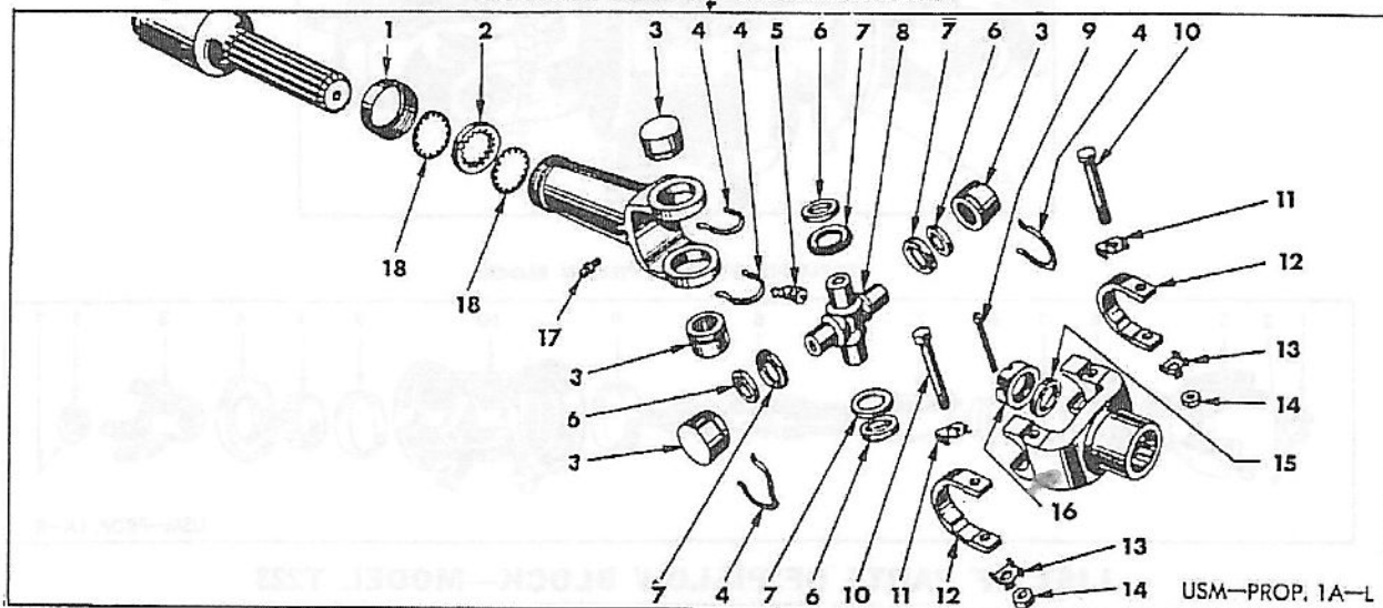
EXPLODED VIEW OF UNIVERSAL JOINT
