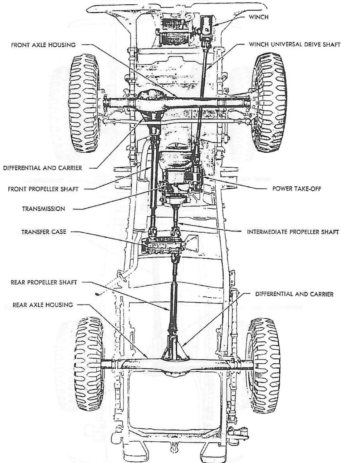
UNDERSIDE VIEW OF CHASSIS MODEL T-214 (4x4)
